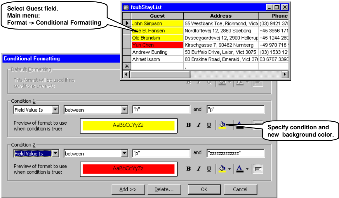
Fig 3.3C Variable colors
