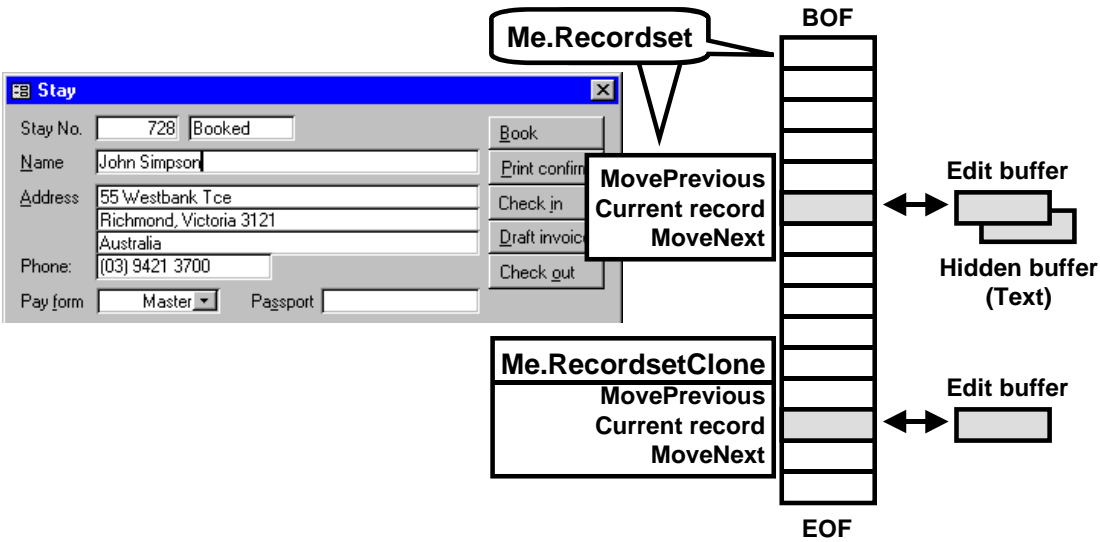
Fig 5.6C Me.Recordset, Me.RecordsetClone
