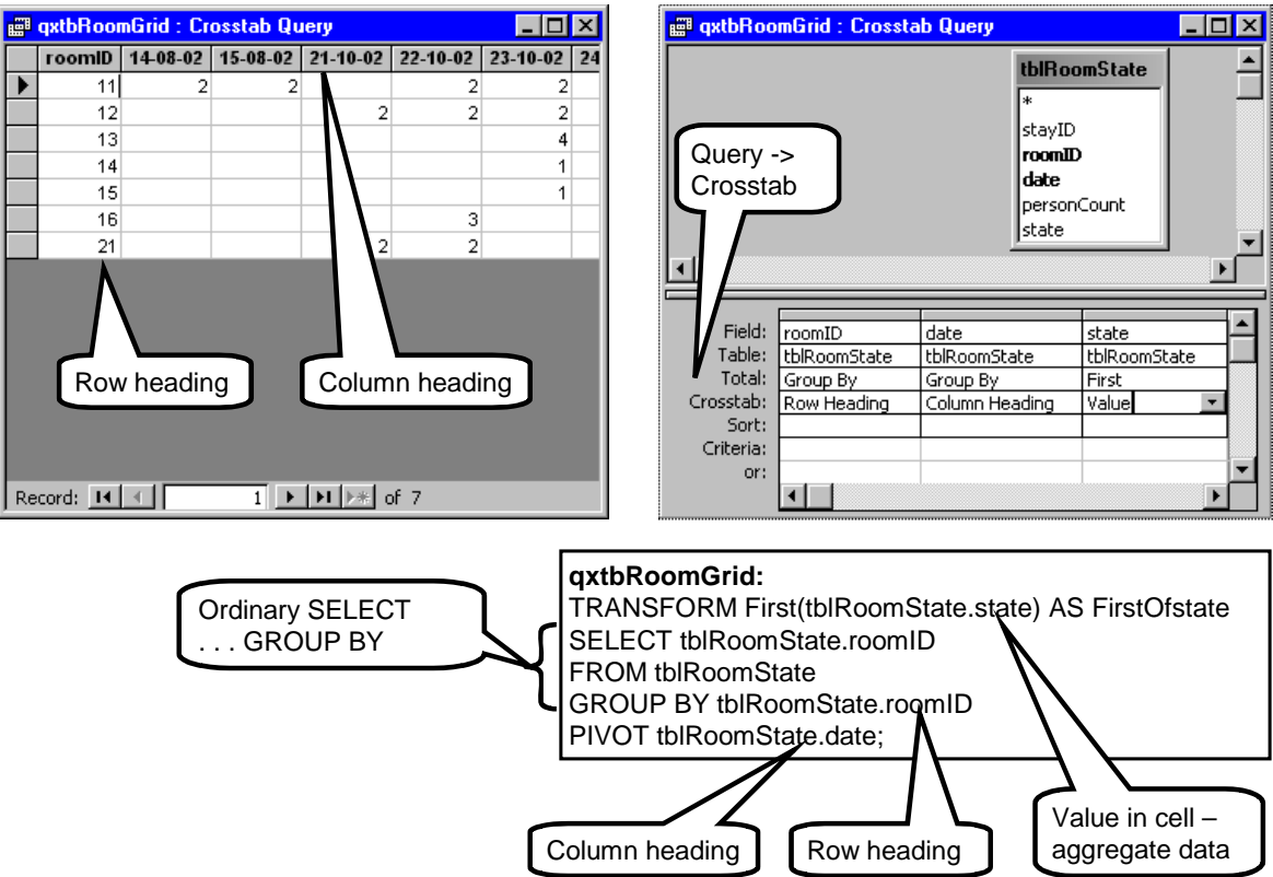
Fig 7.6A Crosstab query
