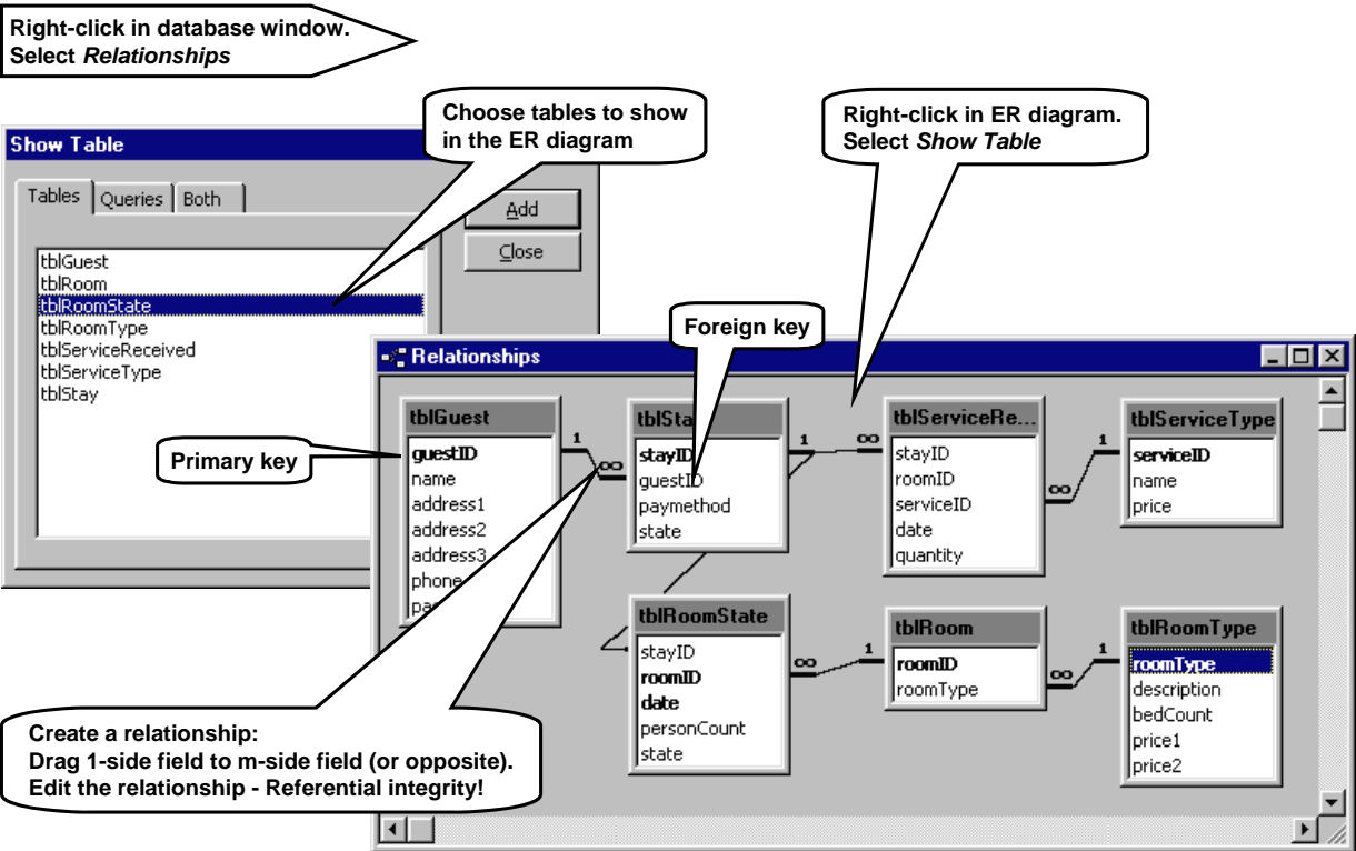
Fig 2.3 Create relationships
