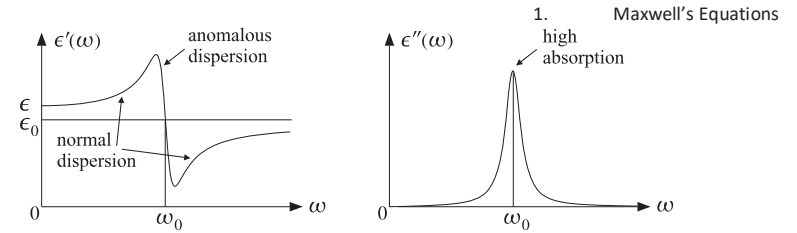
Fig. 1.11.1 Real and imaginary parts of the effective permittivity \epsilon(\omega) .
