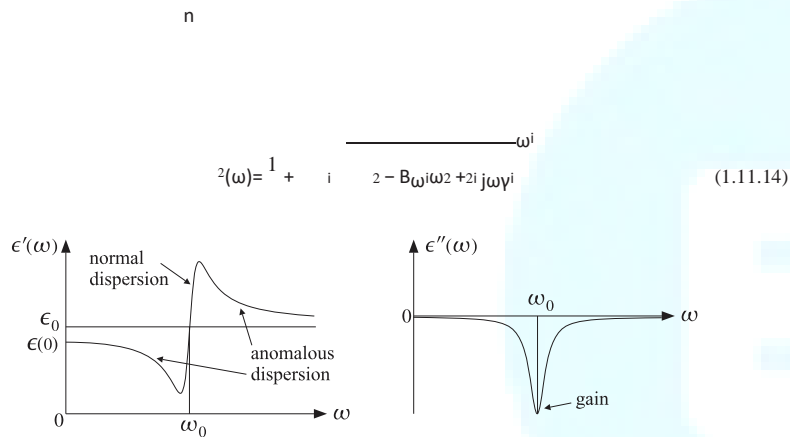
Fig. 1.11.2 Effective permittivity in a two-level gain medium with f = -1 .
