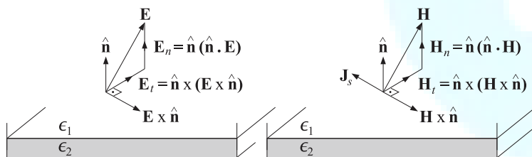
Fig. 1.5.1 Field directions at boundary.
