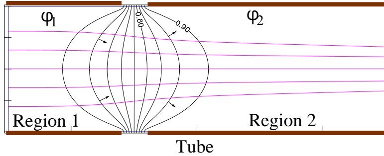
Figure 2.8: The extraction electrode alone always gives a diverging beam.
