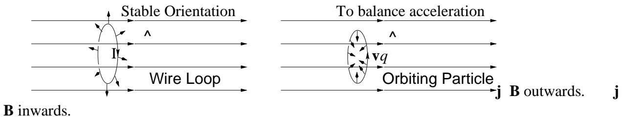
Figure 2.22: Elementary circuit acting as a dipole experiences a force in a non-uniform magnetic field.
