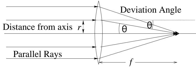
Figure 2.5: Requirement for focussing is that the angular deviation of the path should be a linear function of the distance from the axis.
