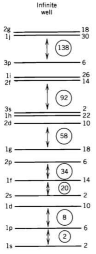
Fig. 2: Shell structure obtained with infinite well and harmonic oscillator potentials. The capacity of each level is indicated to its right. Large gaps occur between the levels, which we associate with closed shells. The circled numbers indicate the total number of nucleons at each shell closure
