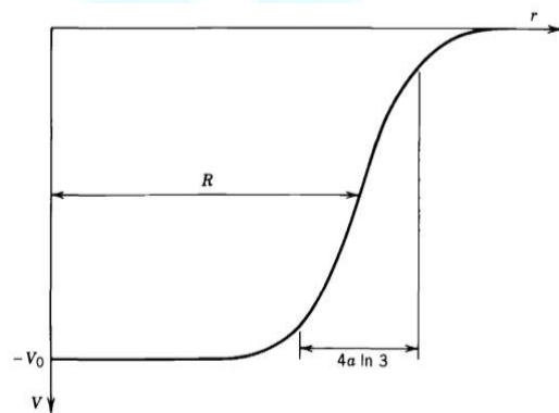
Fig. 3: A realistic form for the shell-model potential.
