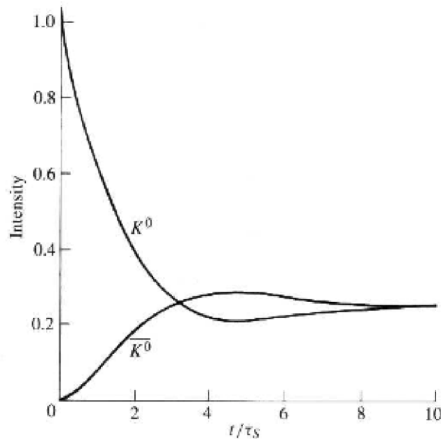
Figure 14.4: Time evolution of an initial K^0 state.
