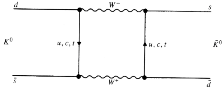
Figure 14.3: A Feynman diagram illustrating the second order weak processing which causes neutral meson mixing. Note that the rate of the mixing is proportional to the CKM matrix elements, e.g. V_{cd}^* V_{cs} .
