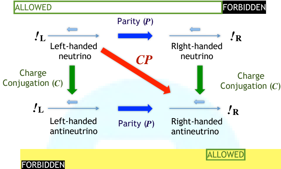
Figure 14.2: The operation of C and P on neutrinos.
