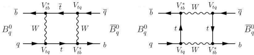
Feynman box diagrams for B mixing.
