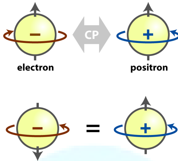
Figure 14.1: The action of the CP (top) and CPT (bottom) operators on a fundamental fermion. The equals sign in the bottom plot represents CPT conservation.
