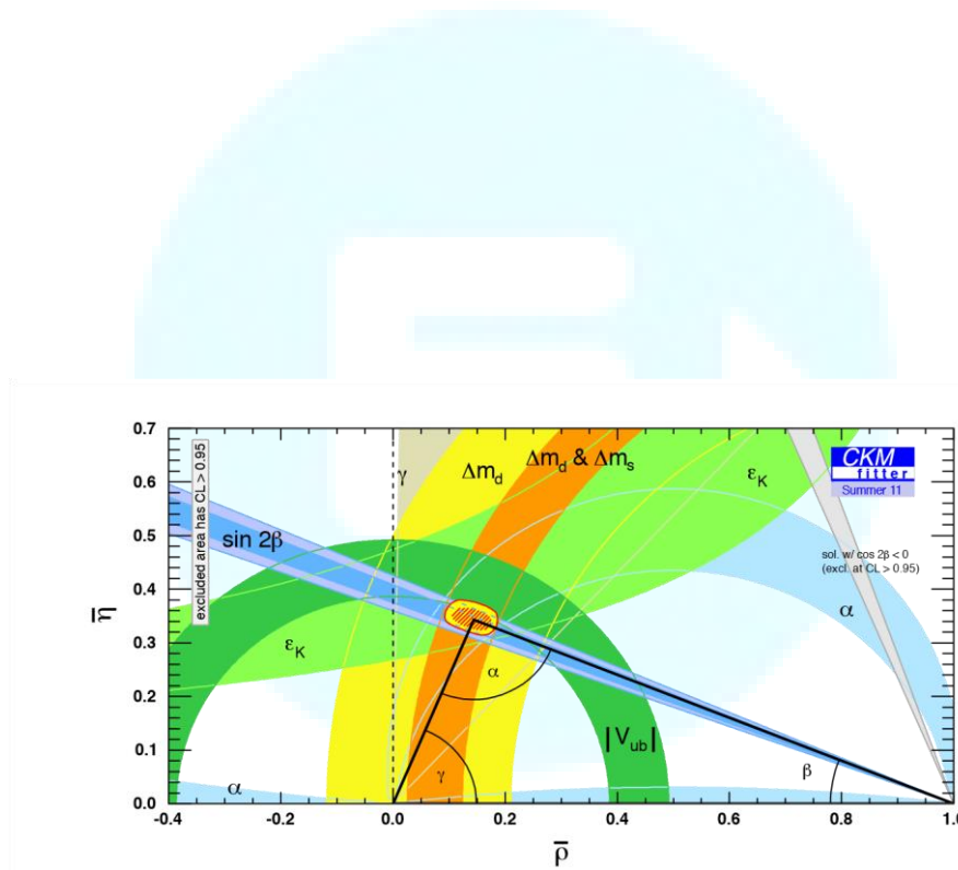
Figure 15.3: Fit of all relevant experimental data to the unitarity triangle parameters.
