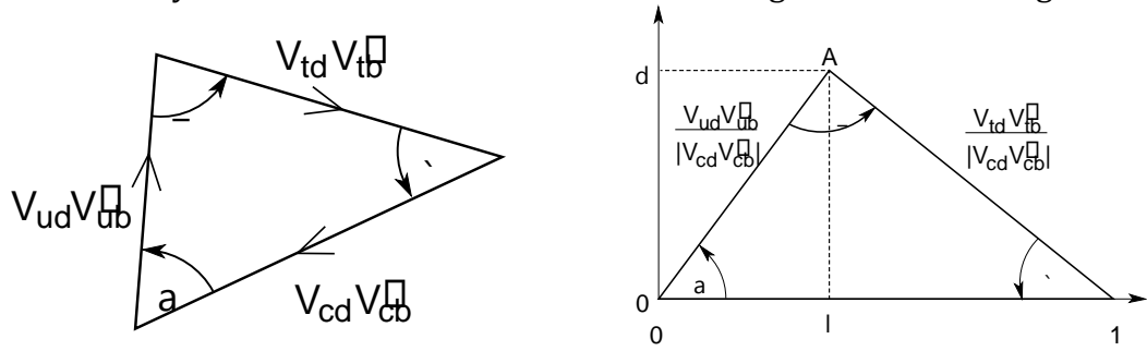
Figure 15.2: Illustration of the unitarity triangle. Left: equation (15.34); right: Dividing through by V_{cd} V_{cb}^* .
